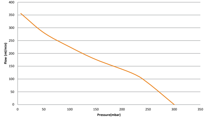
Flow Vs. Pressure (5V DC)
