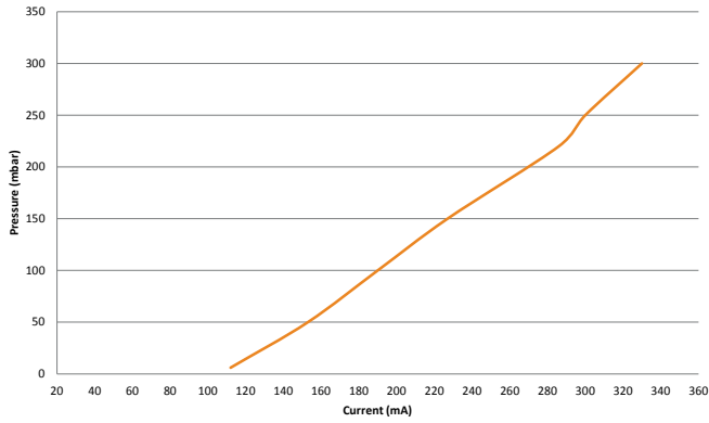
Pressure Vs. Current (5V DC at maximum freeflow)
